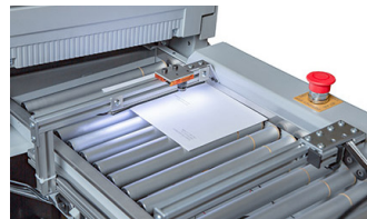
Clear zone detect - rear view
